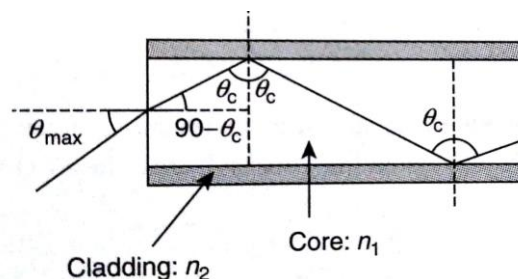
Fig 1.5 : Light Propagation By TIR
