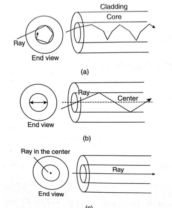
Fig 1.3 : (a) Skew Ray (b) Meridional Ray (c) Axial Ray
