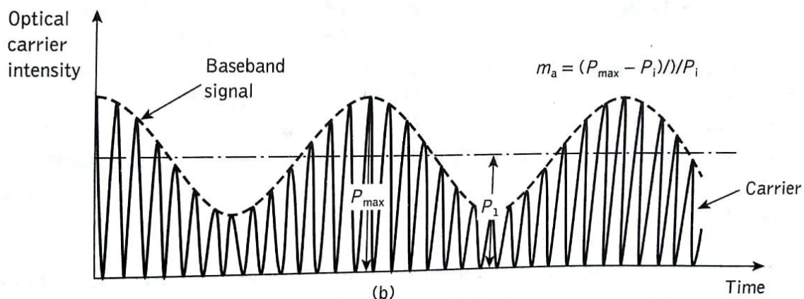
Fig: (a) Analog system employing direct intensity modulation (b) Time domain representation
