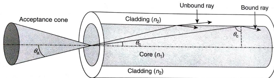
Fig 1.4 : Acceptance cone
