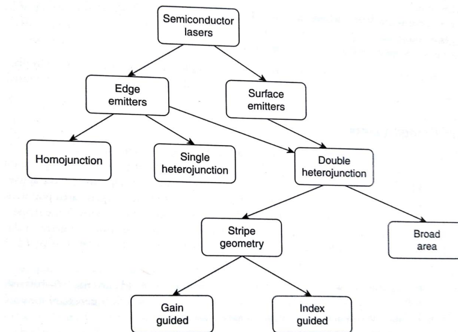
Fig: Classification of laser structures
