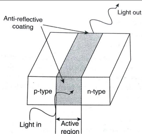
Figure: 5.4 Diagram of SOA
