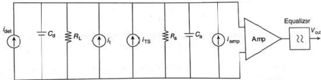
Fig: Equivalent circuit of optical fiber receiver
