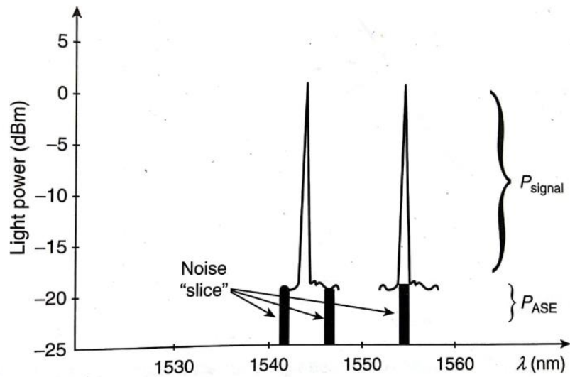
Fig: Noise in EDFA
