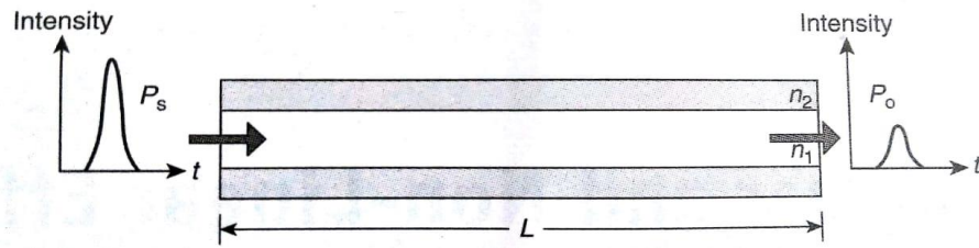
Fig: 1.24 : Attenuation in optical fiber
