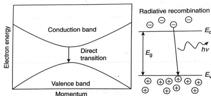
Fig: Direct Bang gap & Direct recombination
