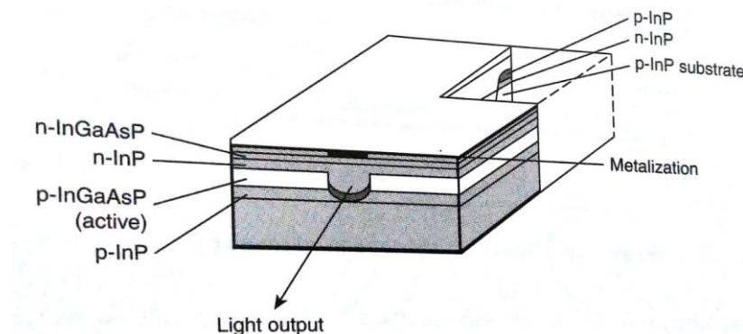
Fig: InGaAsP Super luminescent LED
