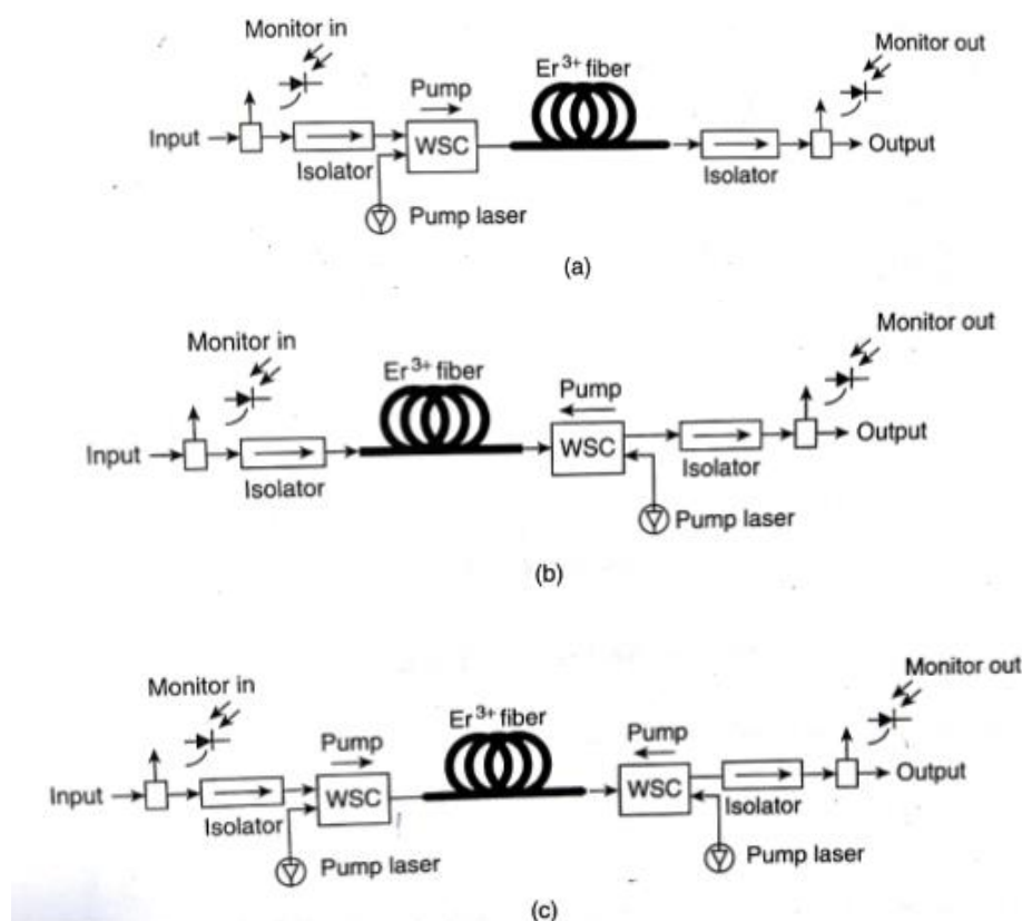
Fig: Different configurations of EDFA. Here WSC is the wavelength selective coupler
