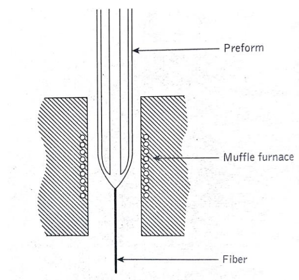
Fig: Optical fiber from a preform
