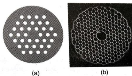
Photonic crystal fibers: (a) Solid core structure and (b) hollow core structure.
