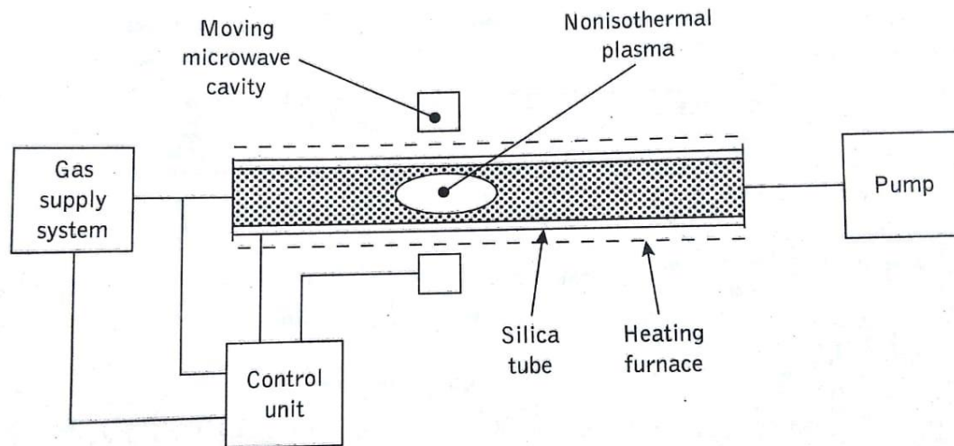
Fig: The apparatus used in PCVD Process
