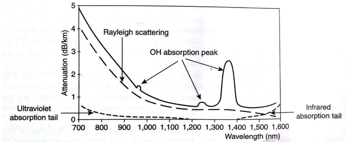
Fig: 1.25 : Fiber Losses
