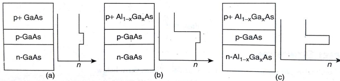
Fig: (a) Homojunction (b) Single heterojunction (c) Double heterojunction
